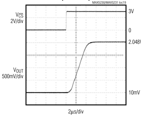
DYNAMIC RESPONSE RISE TIME (MAX5230)
